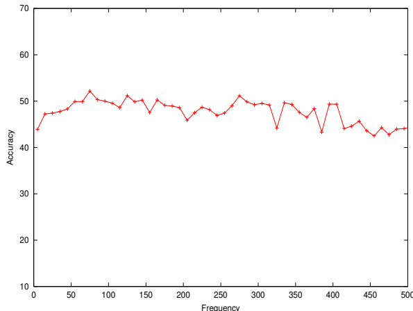
Figure 1: Classification accuracy
